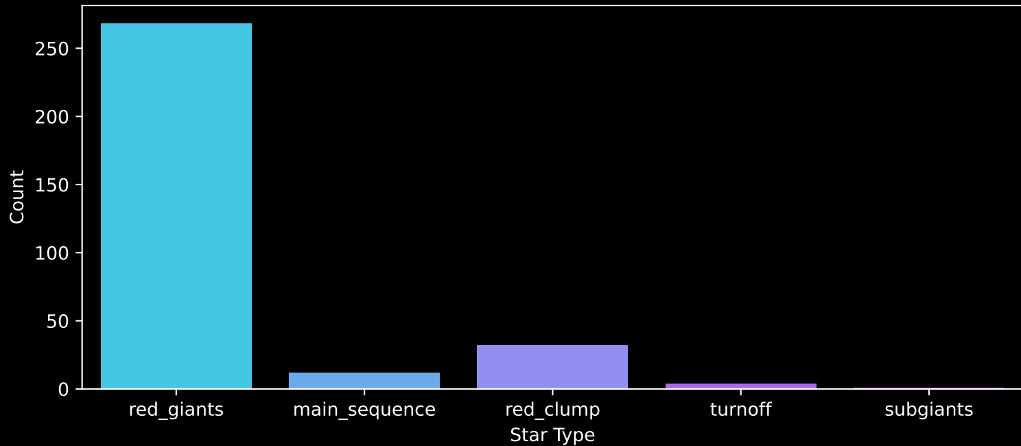
APOGEE DR17 Field: [010+12] Count plot of Star Type
