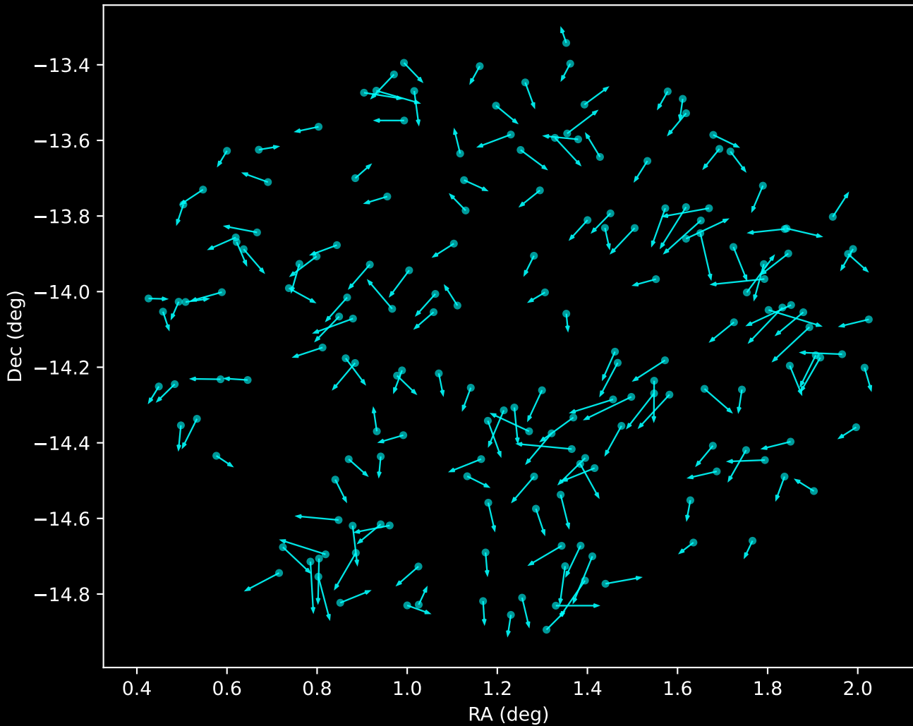
APOGEE DR17 Noise Stream Proper Motion Vectors (n=182)
