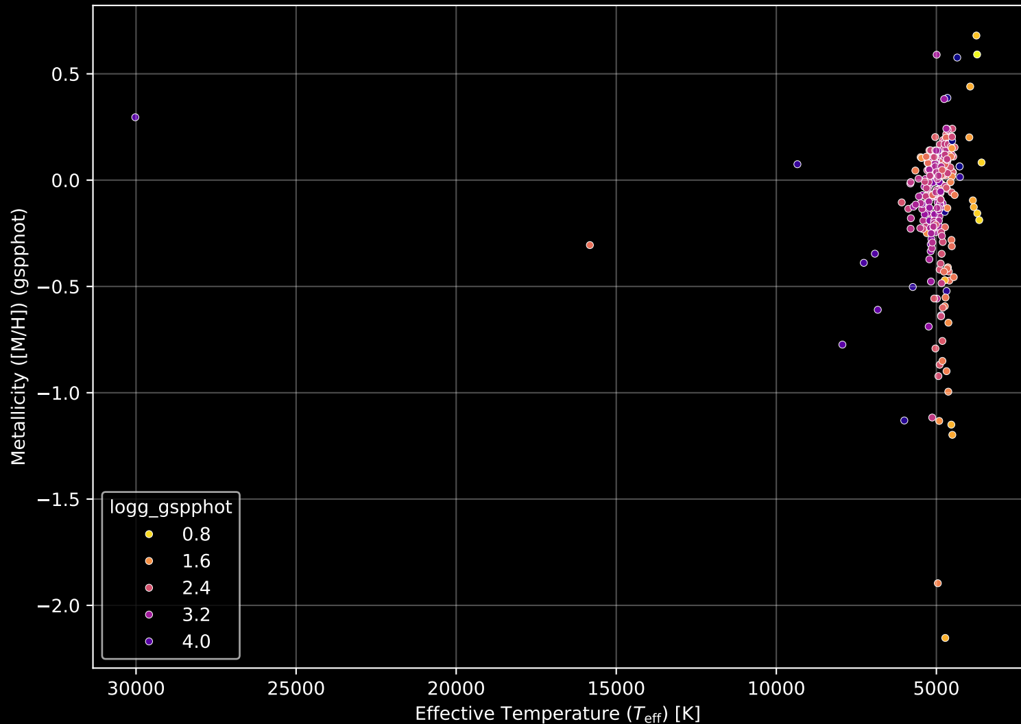
APOGEE DR17 Field: [010+12] Stellar Population Parameters (n= 317)
