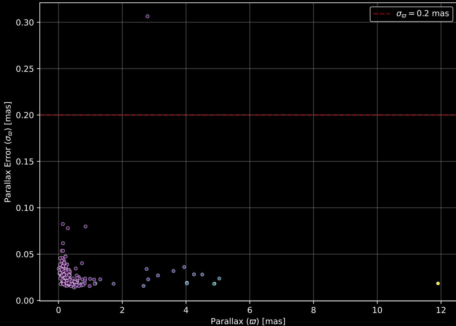
APOGEE DR17 Field: [010+12] Parallax Quality (n= 317)
