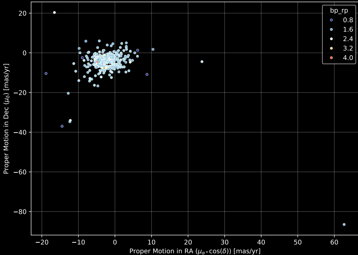
APOGEE DR17 Field: [010+12] Proper Motion Diagram (n= 317)
