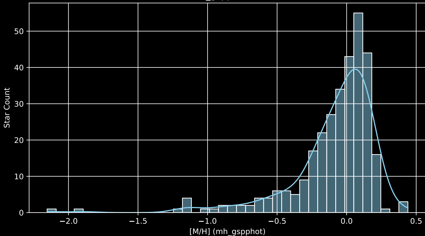
APOGEE DR17 Field: [010+12 [M/H] (mh_gspphot) (n= 313)
