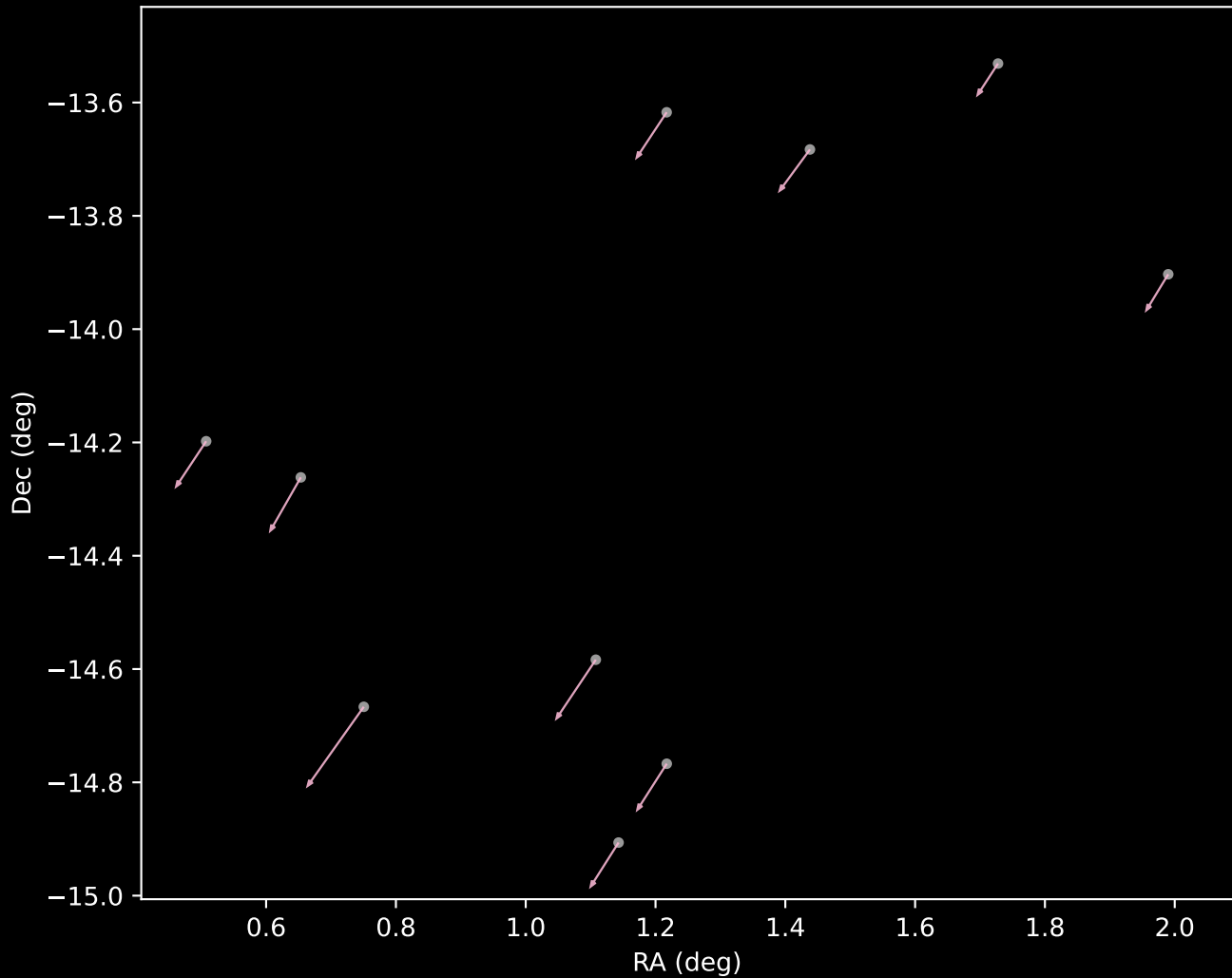
APOGEE DR17 Cluster 13 Proper Motion Vectors (n=10)
