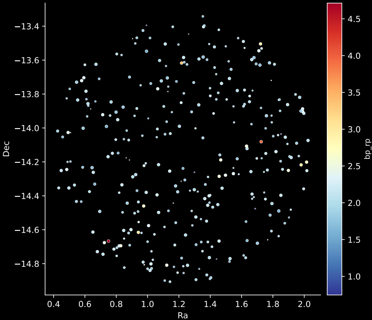
APOGEE DR17 Field: [010+12] Stars: 317
