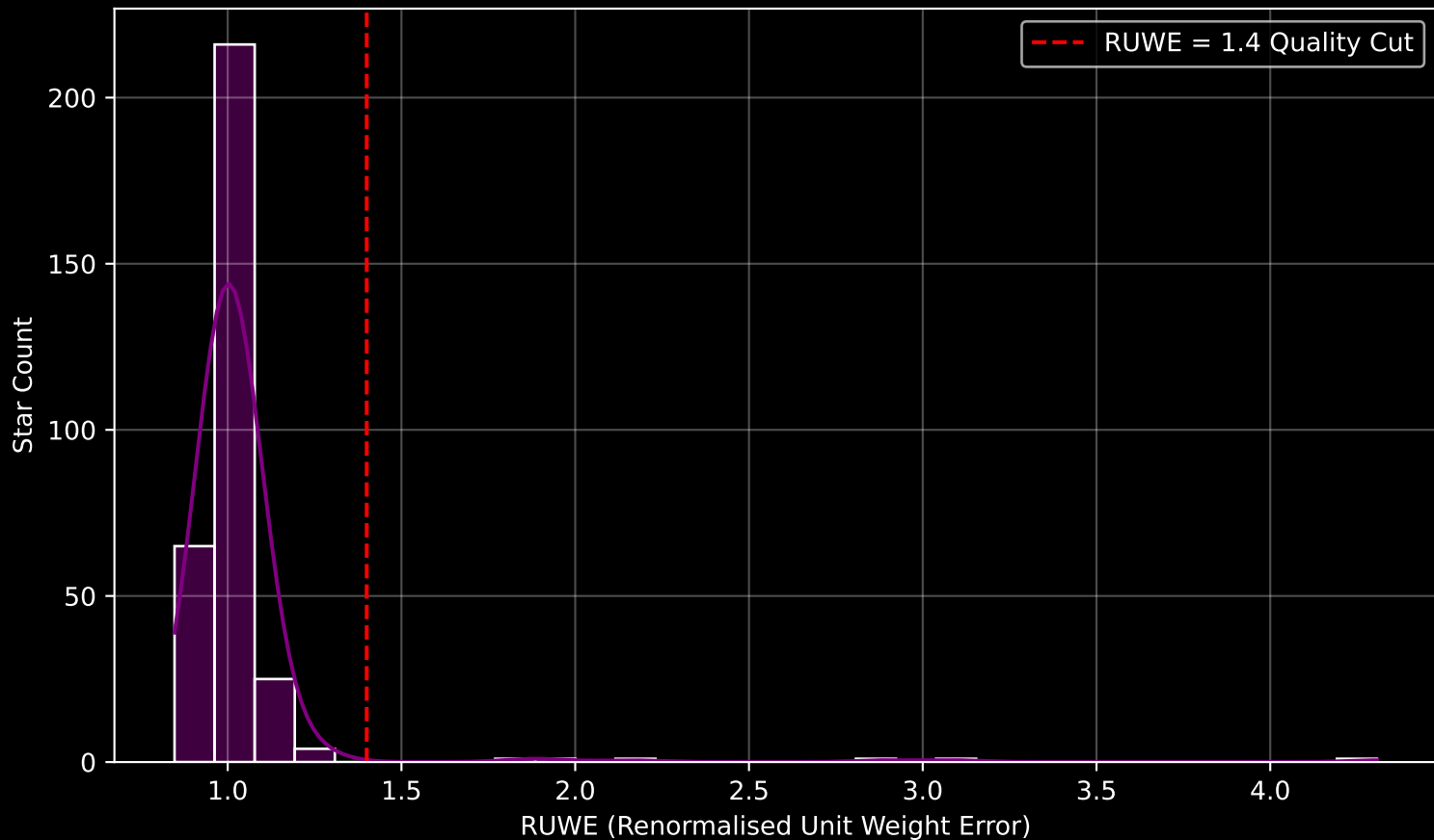
GAPOGEE DR17 Field [010+12] RUWE Distribution (n= 316)
